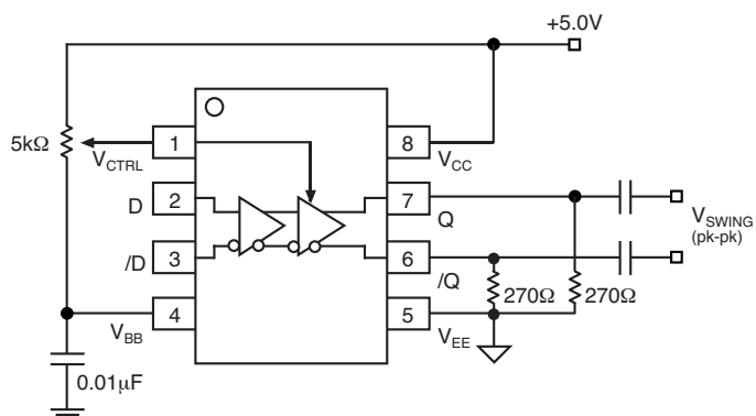
Figure 2. Alternative Implementation
